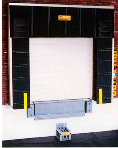
PS-500 Retractable Dock Shelter
